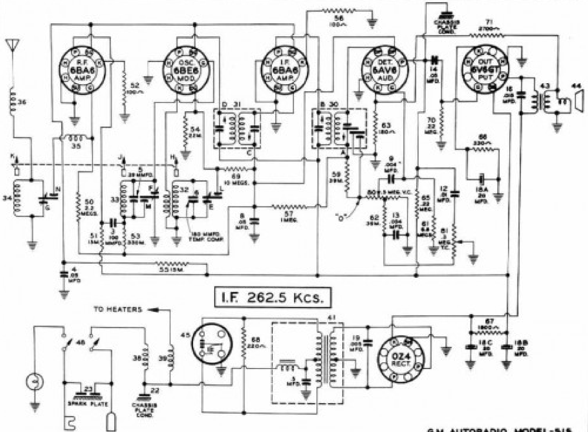
G.M. AUTORADIO MODEL-515 DIAGRAM 5840355
